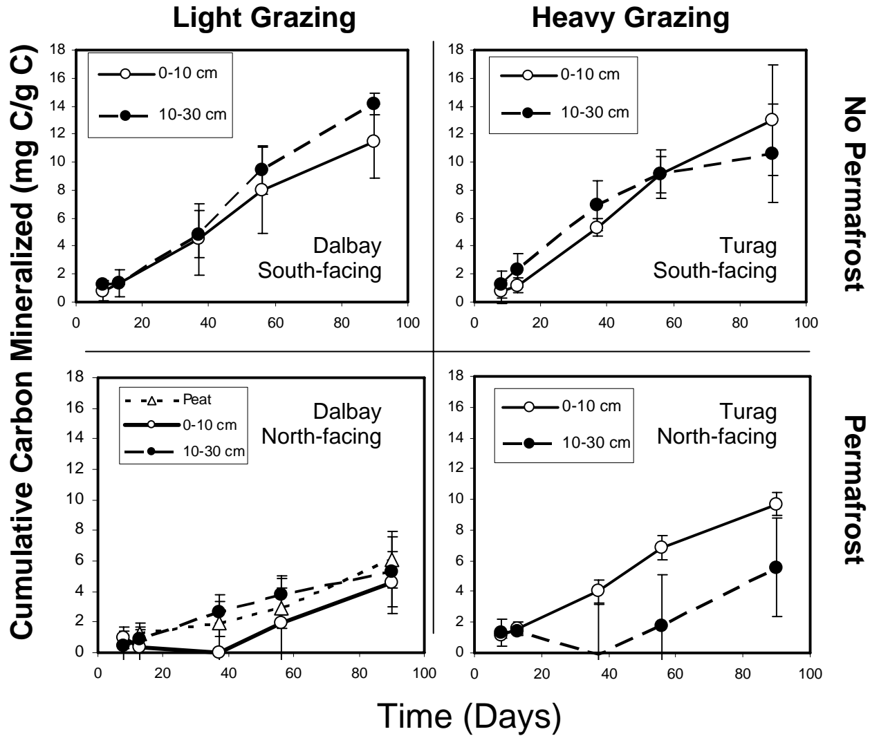
Figure 4 – Cumulative carbon mineralized during the incubations of soils from surface soils (to 30 cm of mineral soil). Only TRG-SL 10-30 showed slowing of decomposition during the 90-day incubation. Error bars are \pm 1 standard error.
